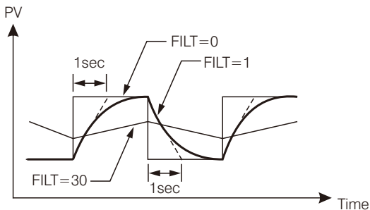
Figure 3-2 Filter Characteristics
