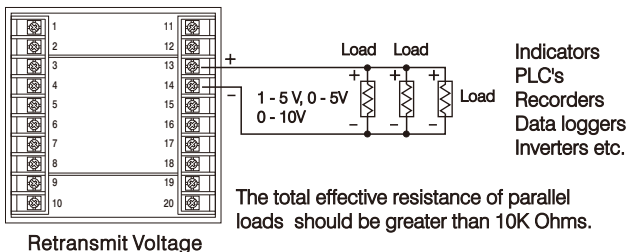
Figure 2-15 Retransmission Wiring
