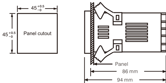
Figure 2-1 Mounting Diagram
