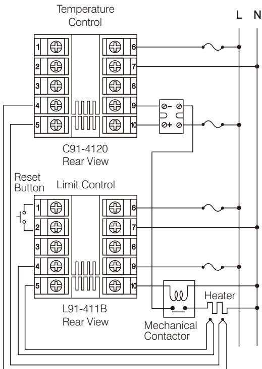
Figure 4-1 Over Temperature Protection with Remote Reset
