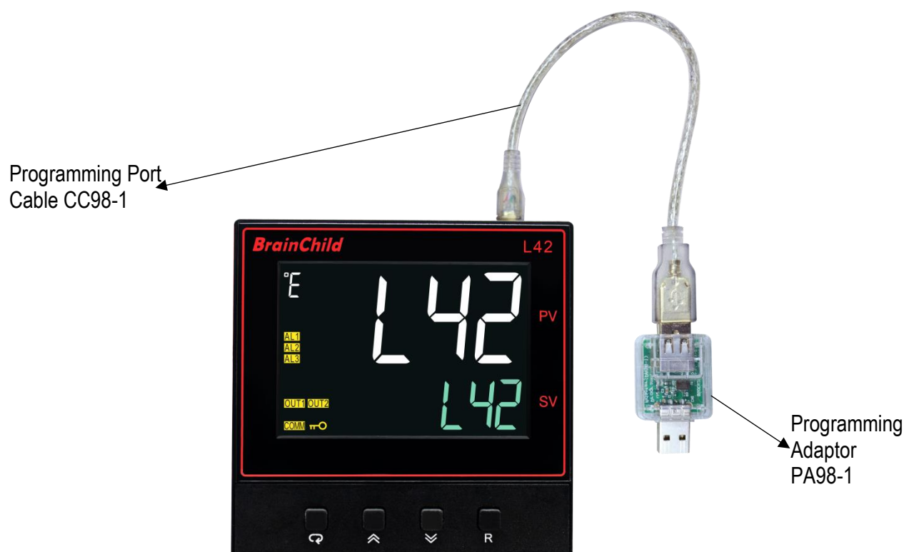
1-2 Programming Port Connection with Programming Port Adaptor
