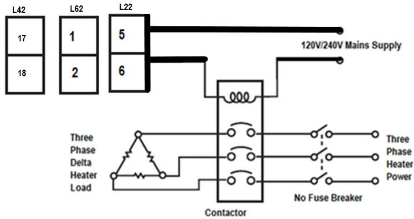
2-18 Output 1 Relay to Drive Contactor
