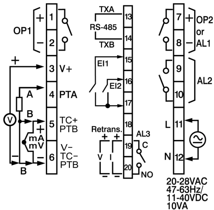
2-10 L62 Rear Terminal Connection – Low Voltage Input Power
