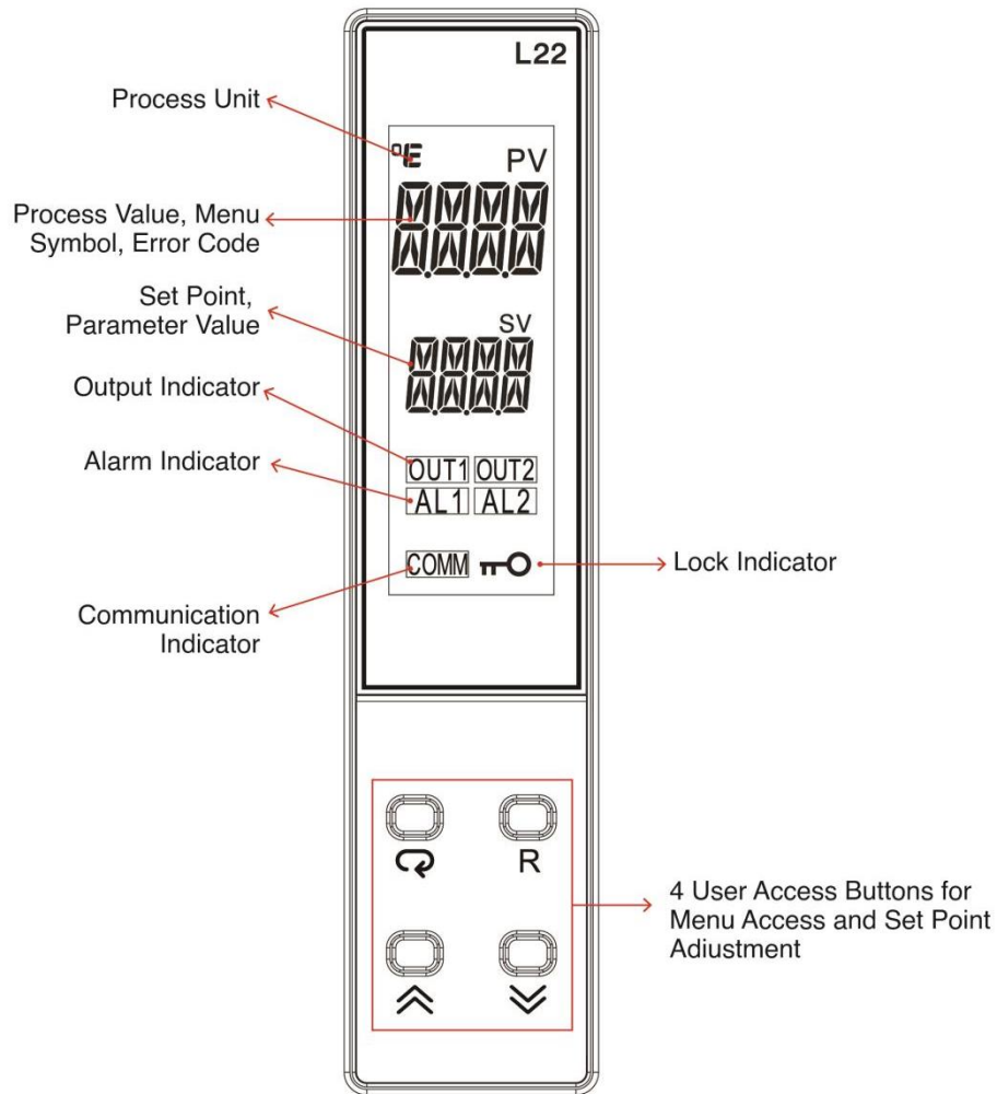
1-5 L22 Front Panel Keys and Display
