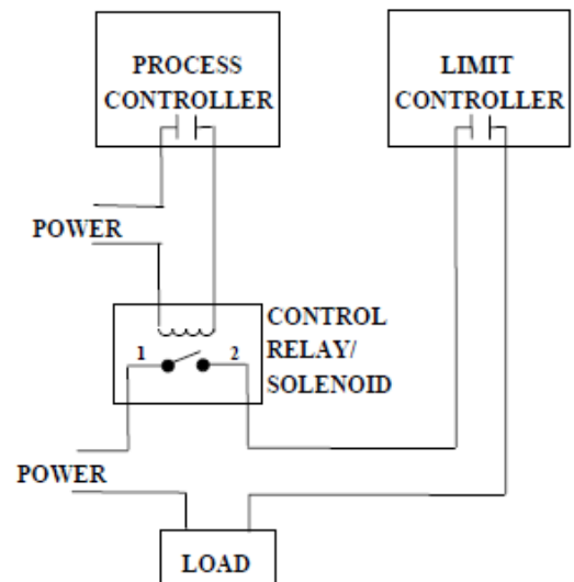
Correct Wiring
