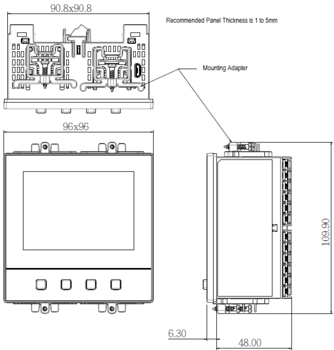
2-1 L42 Dimension with Clamps
