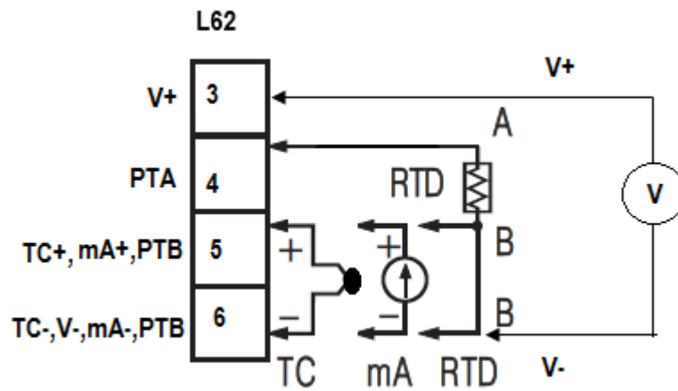
2-15 L62 Sensor Input Wiring
