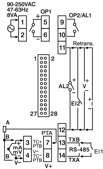
2-11 L22 Terminal Connection– High Voltage Input Power
