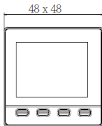
2-4 L62 Dimension without Clamp
