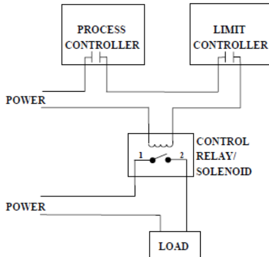
Incorrect Wiring
