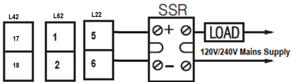
2-19 Output1 Pulsed voltage to Drive SSR
