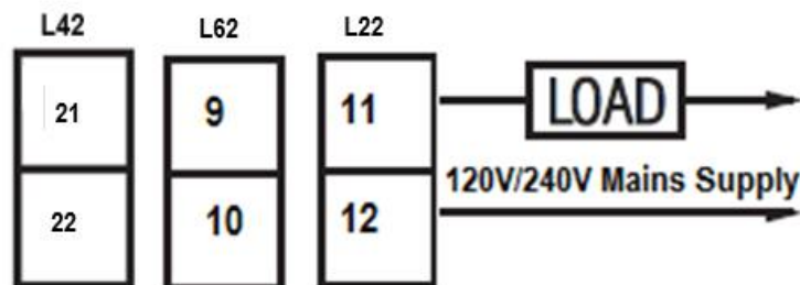
2-21 Alarm 2 Output to Drive Load
