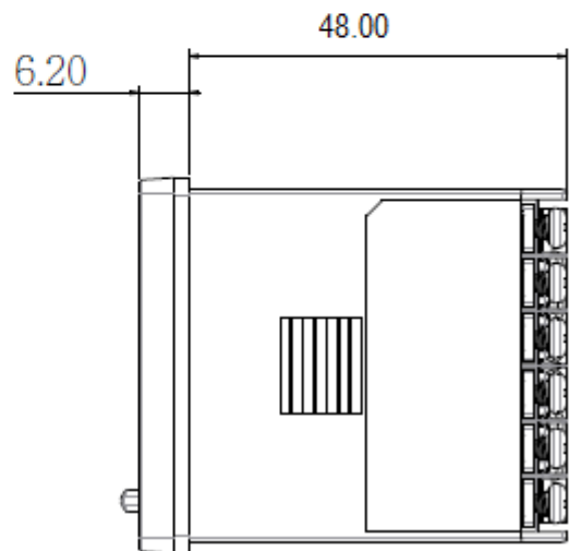
2-4 L62 Dimension without Clamp
