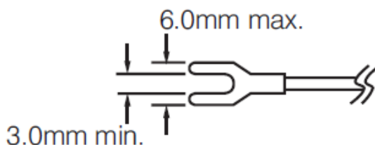
2-6 Lead Terminal
