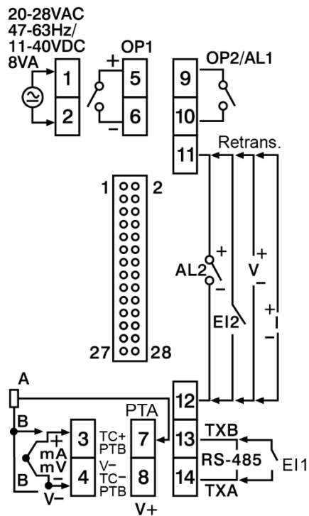
2-12 L22 Terminal Connection– Low Voltage Input Power
