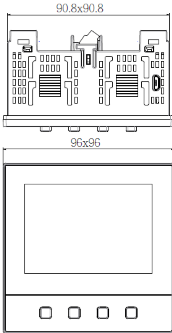
2-2 L42 Dimension without Clamp
