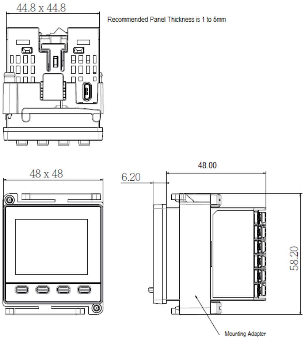
2-3 L62 Dimension with clamp
