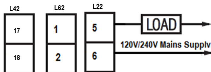
2-17 Output 1 Relay to Drive Load
