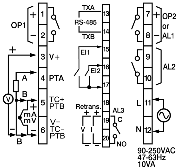
2-9 L62 Rear Terminal Connection – High Voltage Input Power
