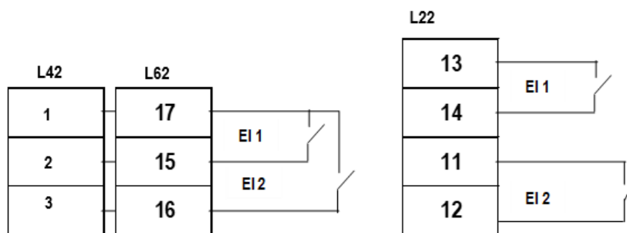
2-23 Event Input Wiring
