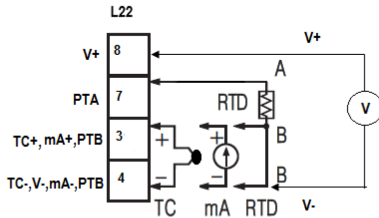
2-16 L22 Sensor Input Wiring
