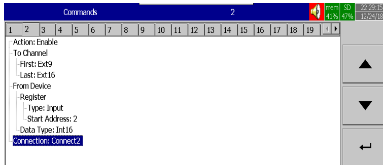
5-22 Mapping of IO Module and External Channel for Slave ID 3
