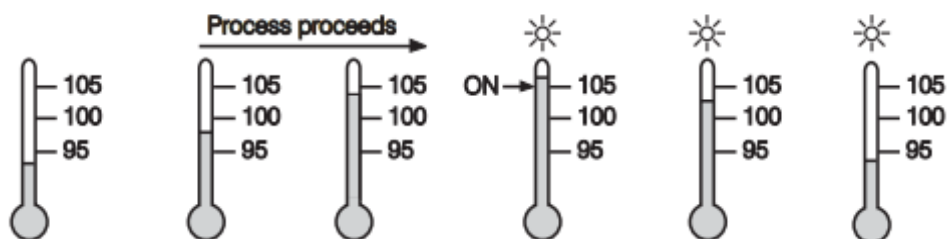
5-12 Latching/Holding Deviation Band Alarm
