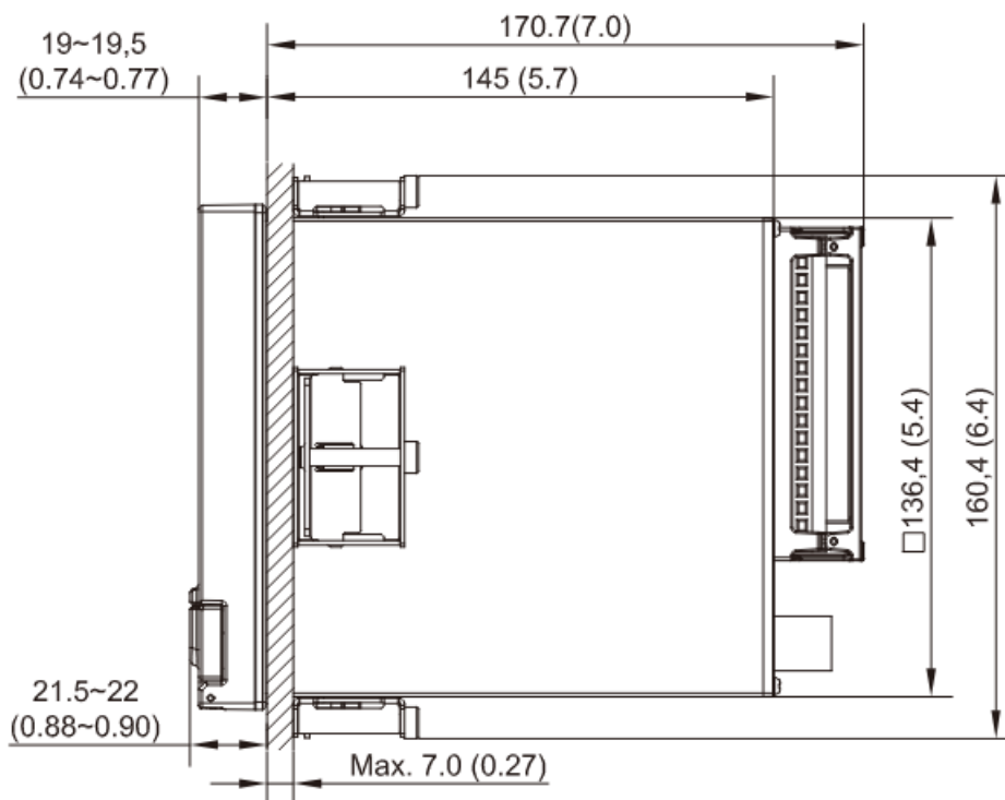
2-5 PR20 Right Side
