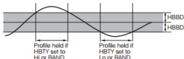
5-13 Holdback on Dwell
