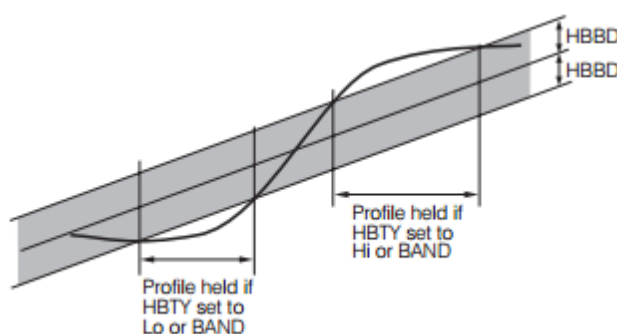
5-14 Holdback on Positive Ramp
