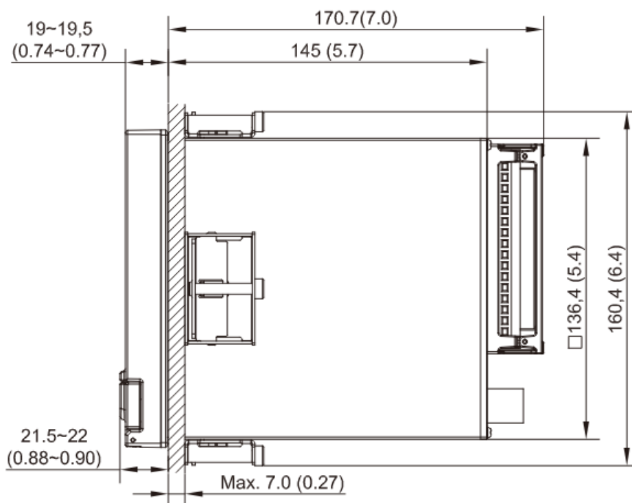
2-2 PR10 Right Side
