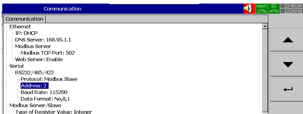
5-40 PR as a Modbus Slave with ID 2
