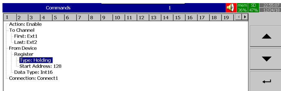
5-35 Mapping of Controller with External Channels
