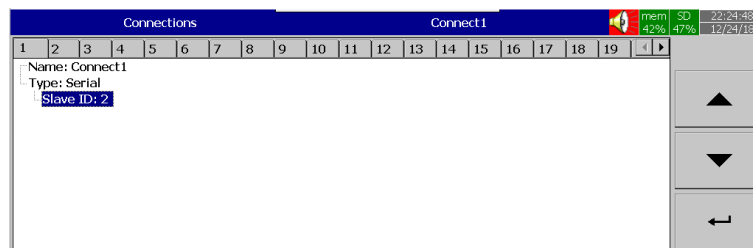
5-19 Connection for Slave ID 2
