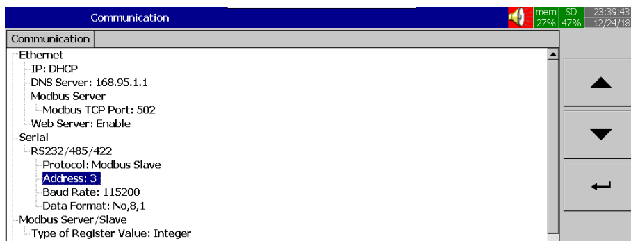
5-41 PR as a Modbus Slave with ID 3
