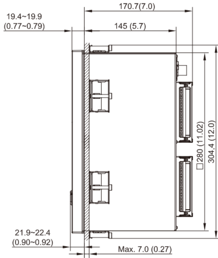
2-8 PR30 Right Side
