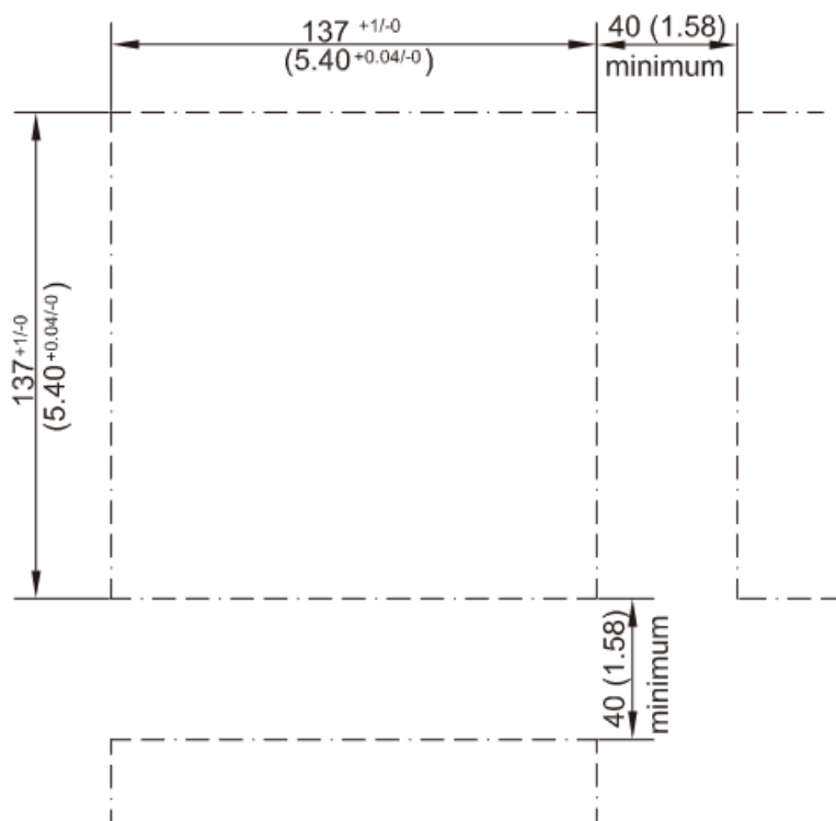
2-6 PR20 Panel Cut-out Dimensions
