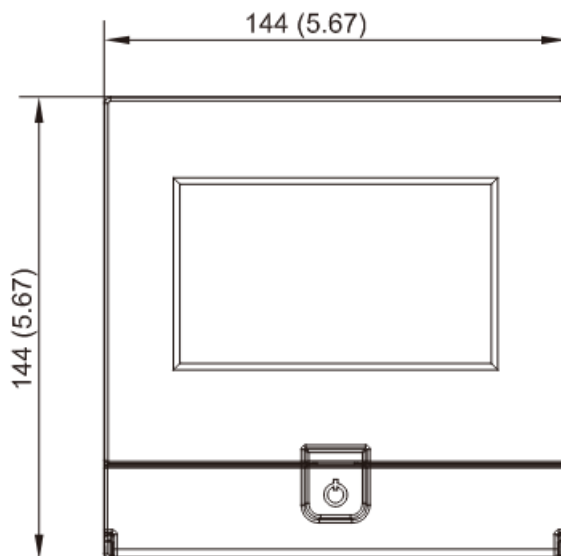
2-1 PR10 Front Side
