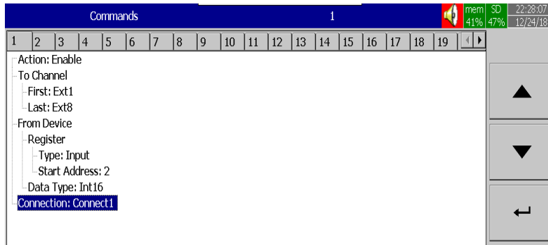
5-21 Mapping of IO Module and External Channel for Slave ID 2
