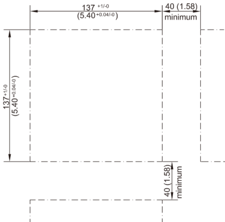
2-3 PR10 Panel Cut-out Dimensions
