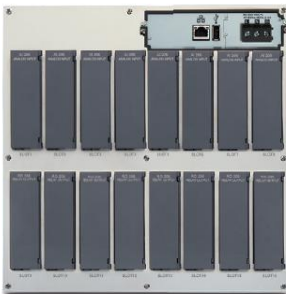
PR30 (16 Slots, up to 48 AI)
