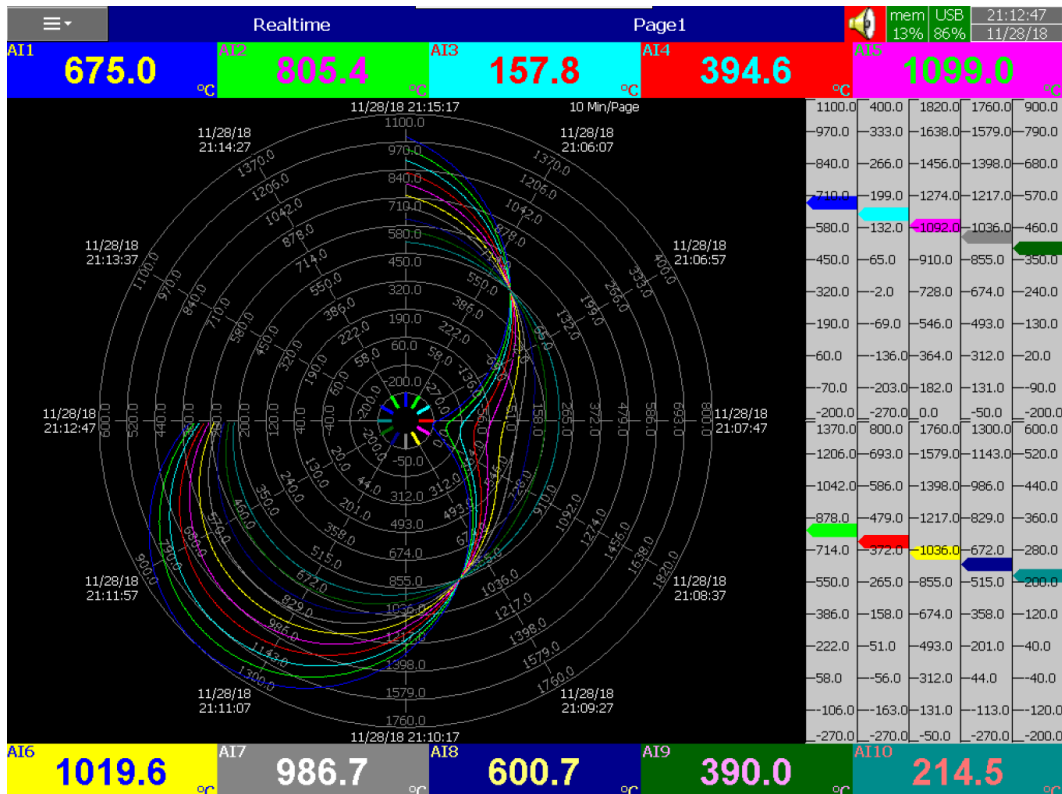
1-5 Circular Chart in PR30
