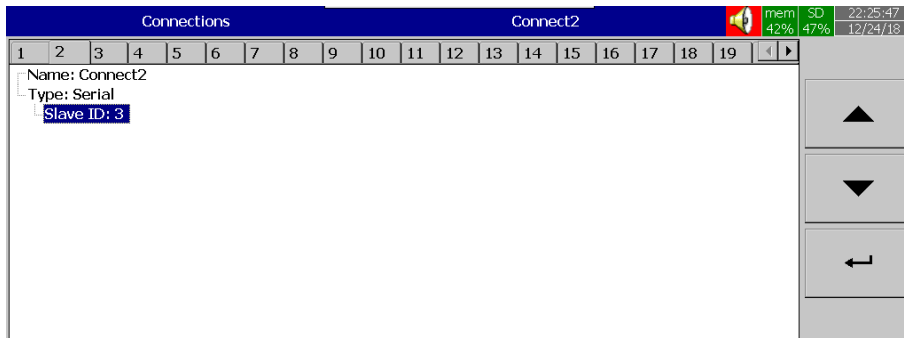
5-24 Connection for Slave ID 3
