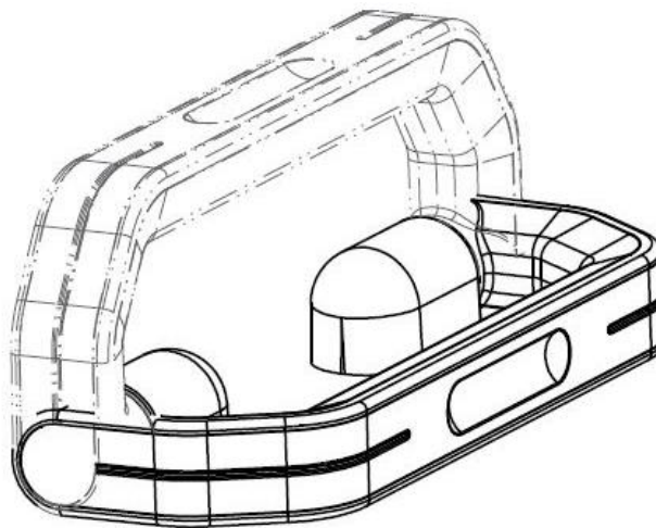
2-15 Portable Type Top Holding Handle
