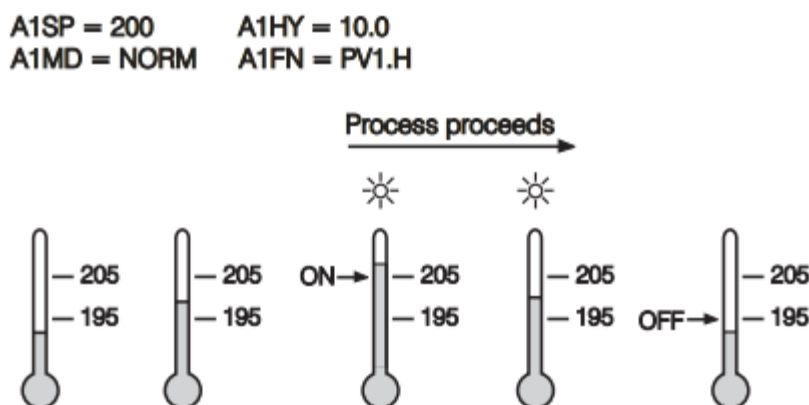
5-1 Normal Process Alarm
