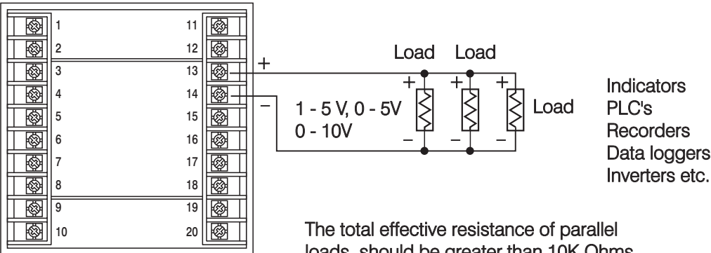
Retransmit Voltage
