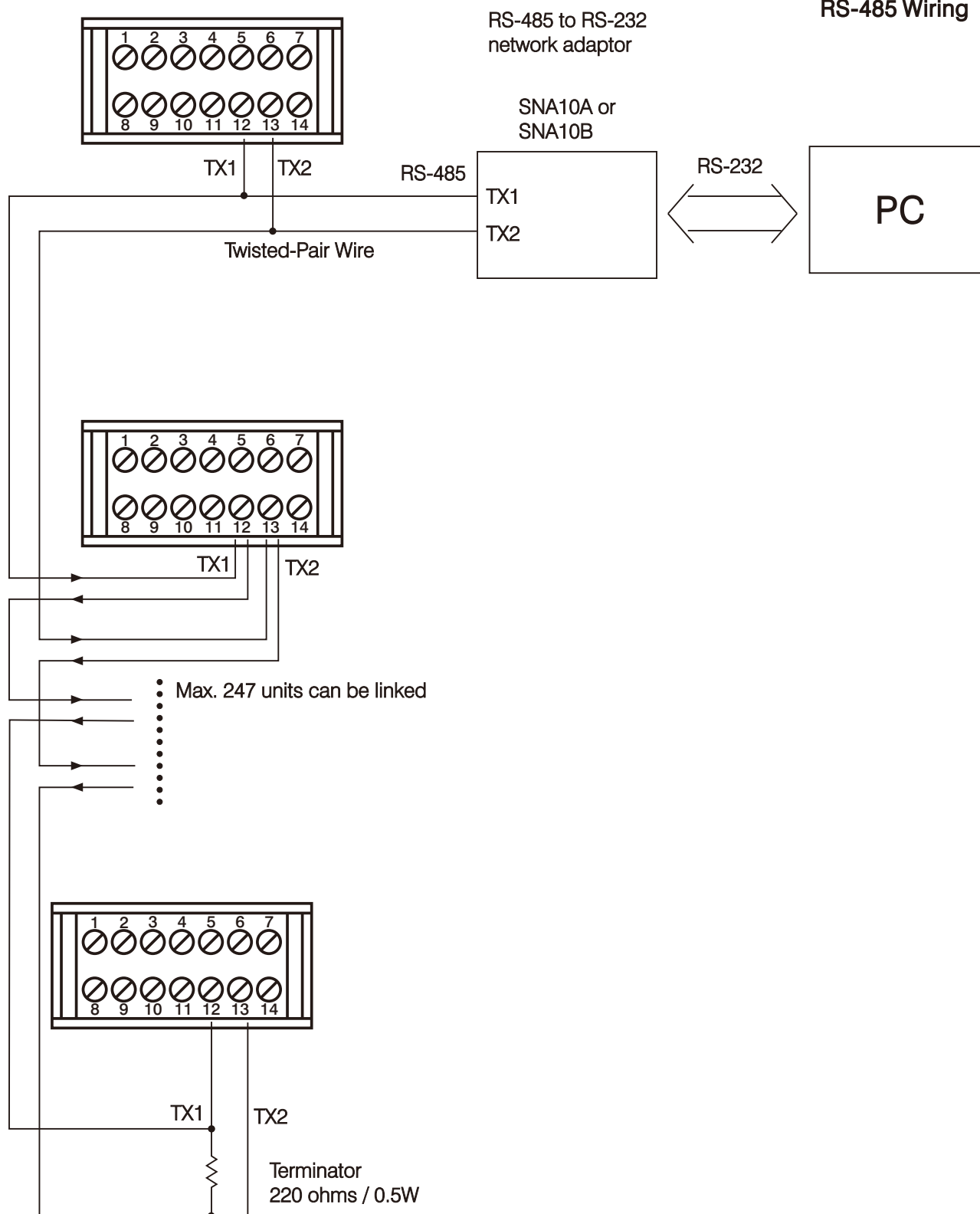
Figure 2.18 RS-485 Wiring
