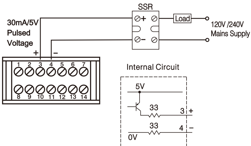
Pulsed Voltage to Drive SSR
