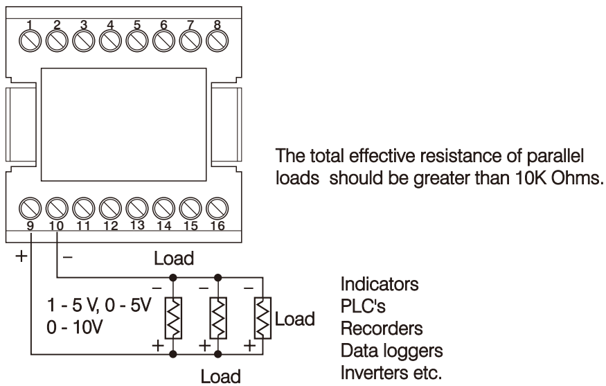
Retransmit Voltage
