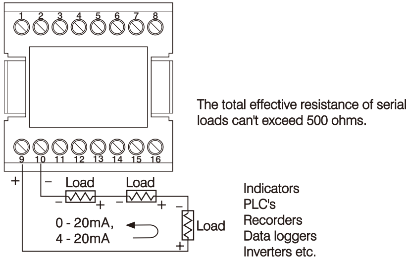
Retransmit Current
