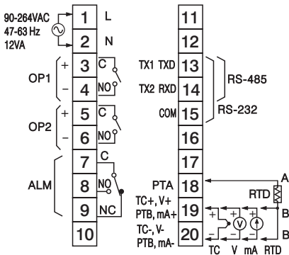
Figure 2.4 Rear Terminal Connection for BTC-4100 and BTC-8100
