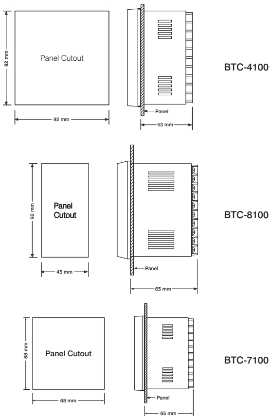
Figure 2.1 Mounting Dimensions
