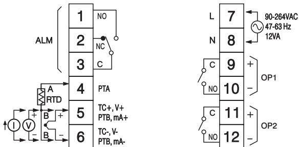
Figure 2.6 Rear Terminal Connection for BTC-9100
