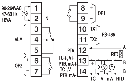
Figure 2.5 Rear Terminal Connection for BTC-7100
