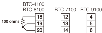
Figure 5.1 RTD Calibration
