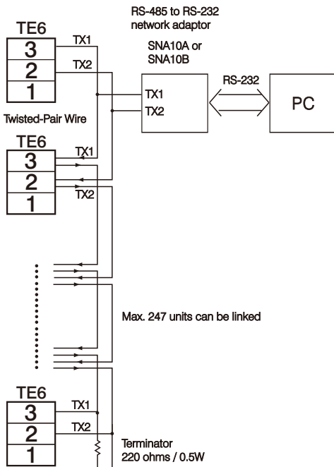
Figure 2.21 RS-485 Wiring
