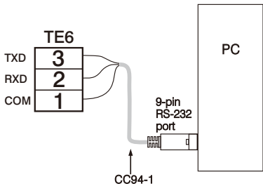
Figure 2.22 RS-232 Wiring
