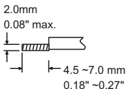
Figure 2.4 Lead Termination
