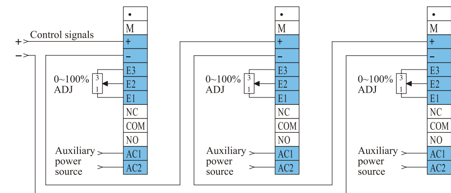
10. Three set connection, independent outside VR setting (limited for 3 sets cascades only)
