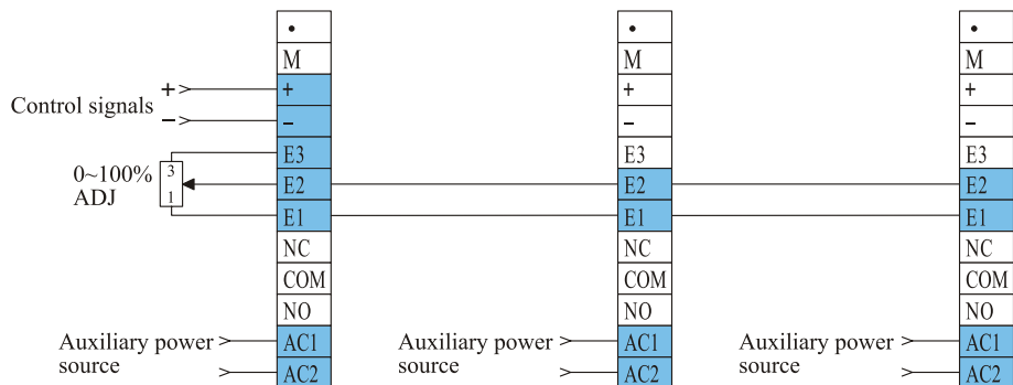
10. Three set connection, independent outside VR setting (limited for 3 sets cascades only)
